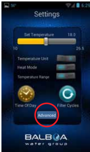
SETTINGS SCREEN
