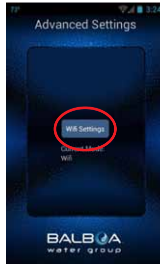
ADVANCED SETTINGS
